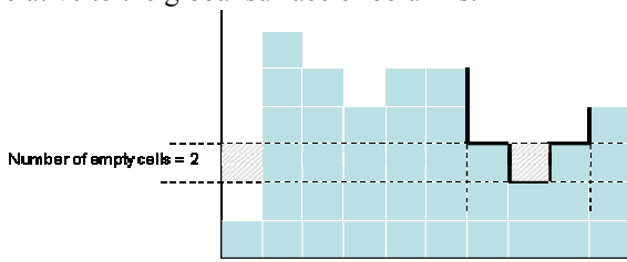
Figure 4 – Degree of intrusion. This corresponds to the number of empty cells at the bottom of the pattern.
